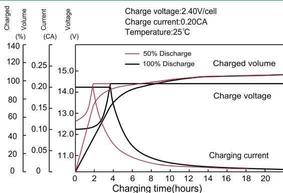
Charge characteristic curve
